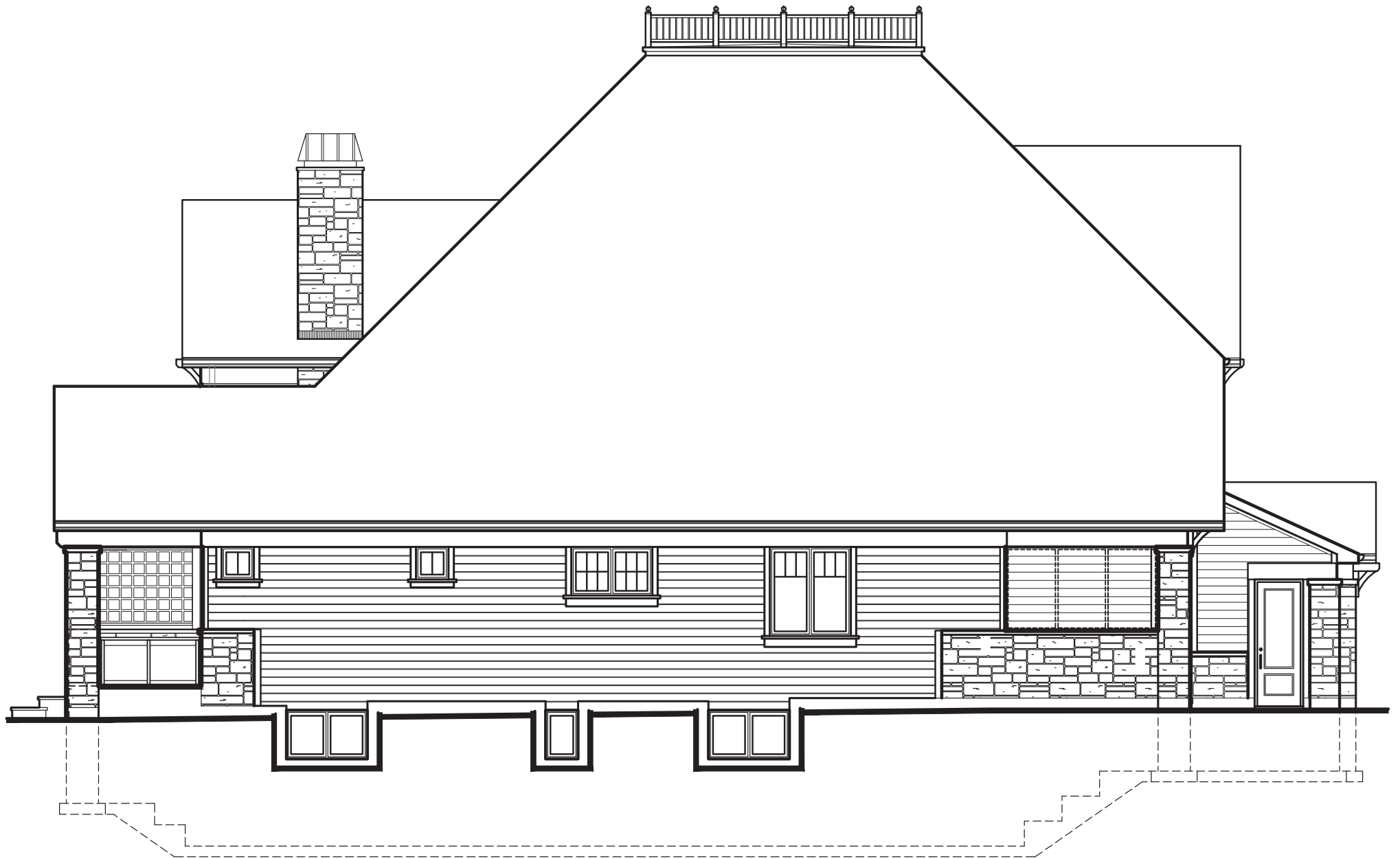
The Muirfield Left Side Elevation
